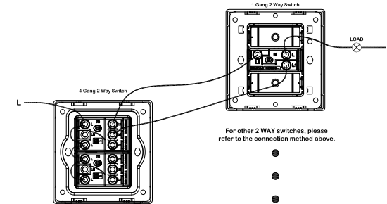
4 Gang 2 Way Switch
