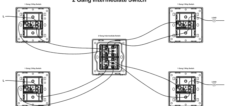
2 Gang Intermediate Switch
