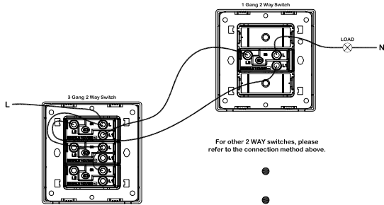
3 Gang 2 Way Switch
