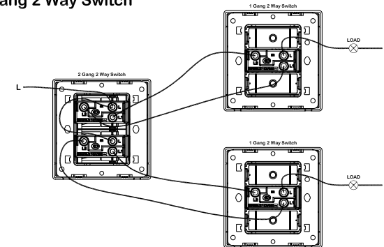
2 Gang 2 Way Switch
