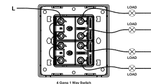
4 Gang 1 Way Switch
