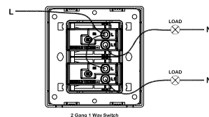
2 Gang 1 Way Switch
