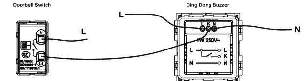
Doorbell Switch with Ding Dong Buzzer.
