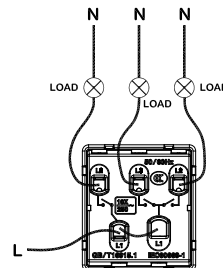
3 Gang 1 Way Switch
