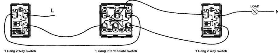
1 Gang 2 Way Switch
