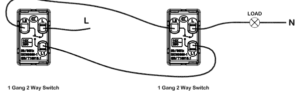
1 Gang 2 Way Switch
