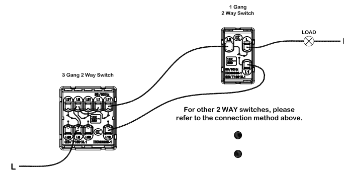
3 Gang 2 Way Switch
