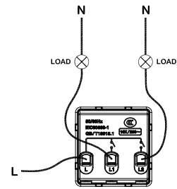
2 Gang 1 Way Switch
