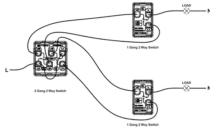
1 Gang 2 Way Switch
