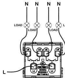
4 Gang 1 Way Switch
