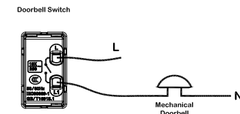
Doorbell Switch with Mechanical Doorbell.
